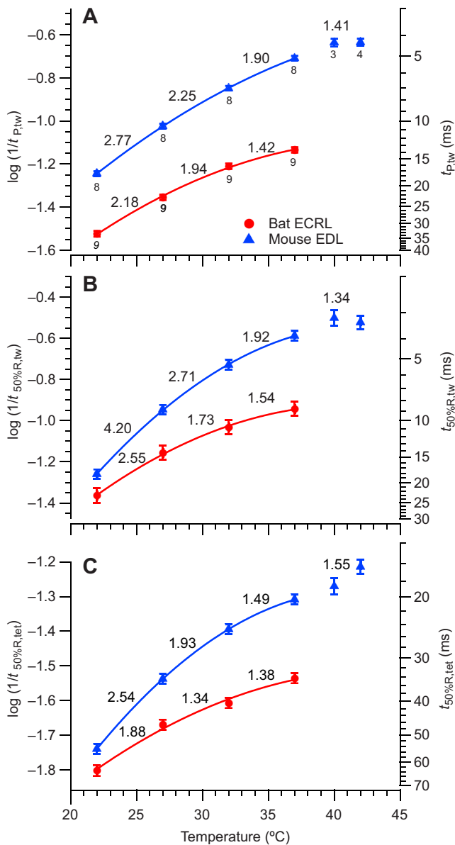
Fig. 3. log of inverse contraction times ( \text{ms}^{-1} ) as a function of temperature for the ECRL of the bat C. perspicillata and the EDL of the laboratory mouse. (A) Time to peak force in a twitch ( t_{P,tw} ). (B) Time from peak force to 50% relaxation in a twitch ( t_{50\%R,tw} ). (C) Time from peak force to 50% relaxation in a tetanus ( t_{50\%R,tet} ). The points plotted are the mean values at each temperature ( \pm s.e.m.); sample sizes for the means are indicated below each point in A. The solid lines are quadratic regressions fitted using the individual log-transformed values at temperatures of 37°C and below ( n =the sum of the sample sizes at each temperature). The numbers above the curves indicate the Q_{10} values calculated for 5°C intervals. The right axes show the times on an inverted log scale.
