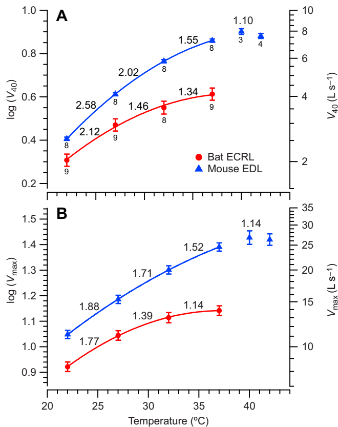
Fig. 5. log-transformed shortening velocity as a function of temperature for the ECRL of the bat C. perspicillata and the EDL of the laboratory mouse. (A) Shortening velocity at 40% of maximum force ( V_{40} , in L s -1 ). (B) Predicted maximum shortening velocity at zero force ( V_{max} , in L s -1 ). The points plotted are the mean values at each temperature ( \pm s.e.m.); sample sizes for the means are indicated below each point in A. The solid lines are quadratic regressions fitted using the individual log-transformed values at temperatures of 37°C and below ( n =the sum of the sample sizes at each temperature). The numbers above the curves indicate the Q_{10} values calculated for 5°C intervals. The right axes show velocity on a log scale.
